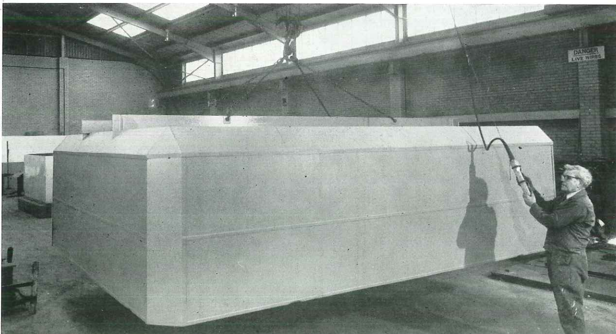
A typical lift off cover type furnace for in-house heat treatment of drilling tubes, modular pipe work and grey iron castings being lowered into position.
